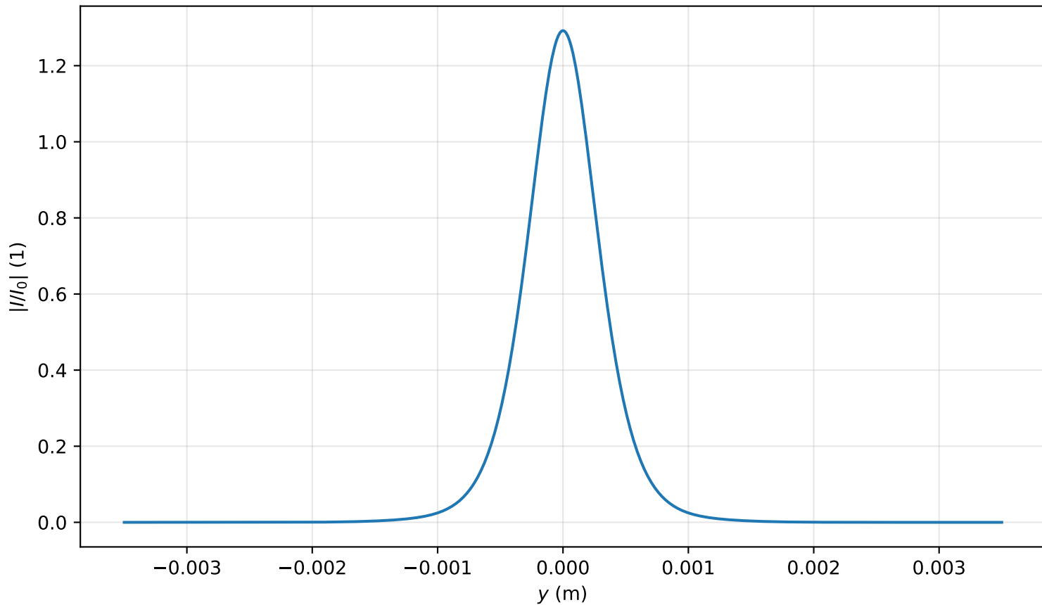
Intensity profile I(x=0, y, z=2.149)/I_0 , P_{in}=0.8P_{cr} , artificial time
